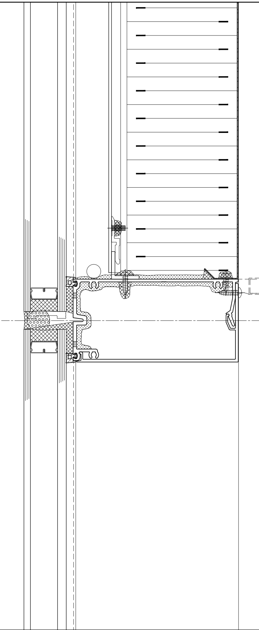
① TYPICAL SECTION DETAIL @ HORIZONTAL TRANSOM
